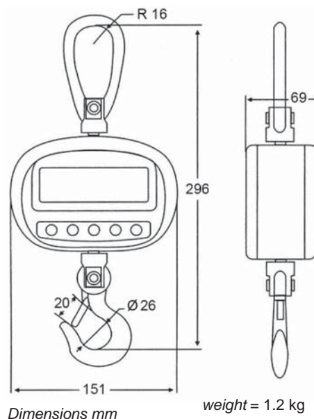
Dimensions mm
