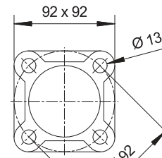
Flange dimensions
